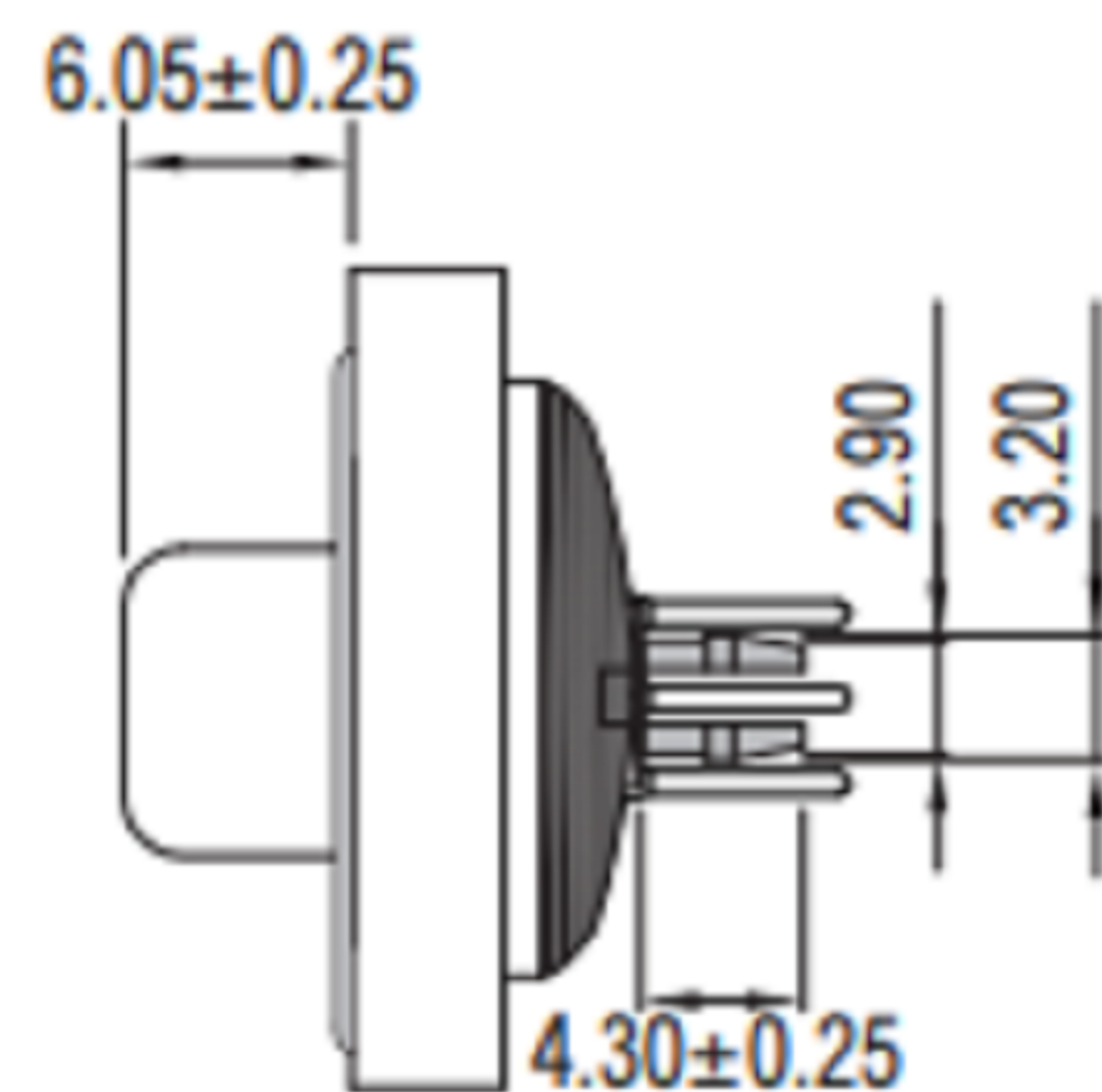
直式孔型插座(焊板式, 定位柱) EDB4 Straight Female Socket(PCB, Peg) EDB4 - F 37 - PPA 14 - DW
